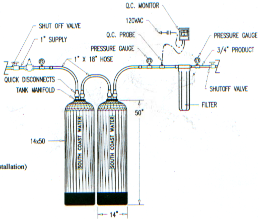
(2X) 14 x 50 TANKS MANIFOLDED
